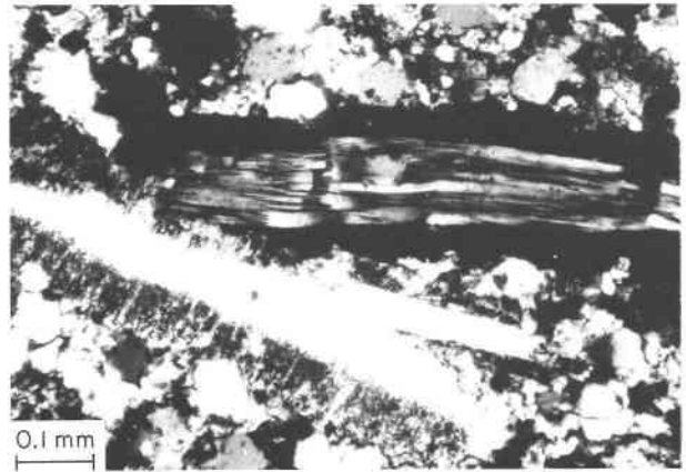
Fig. 2. Photomicrograph showing deformed polysynthetic twinning in albite phenocryst rimmed by potassium feldspar (at extinction), and cloudy potassium feldspar rimming clear albite phenocryst.
