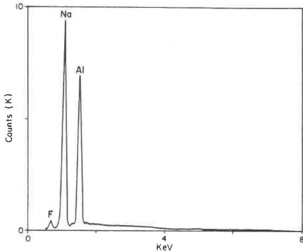
Fig. 6. Energy-dispersive spectrum of cryolite ( \text{Na}_3\text{AlF}_6 ).
